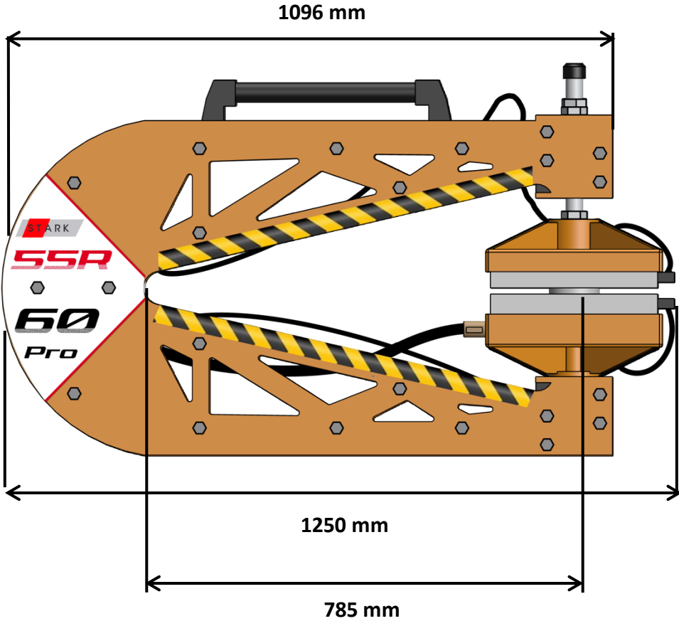
SIDE VIEW
