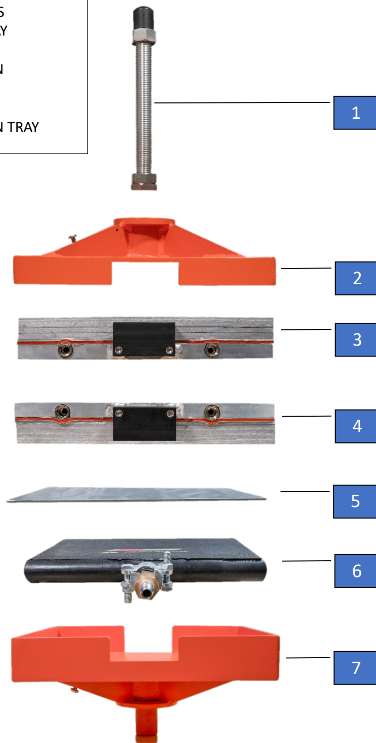
SPOT REPAIR PLATEN ASSEMBLY (EXPLODED VIEW)
